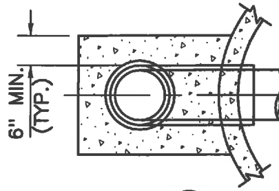
SECTION (A)
