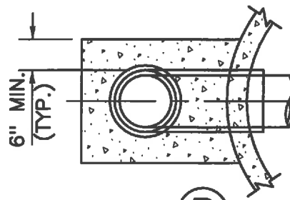
SECTION (B)
