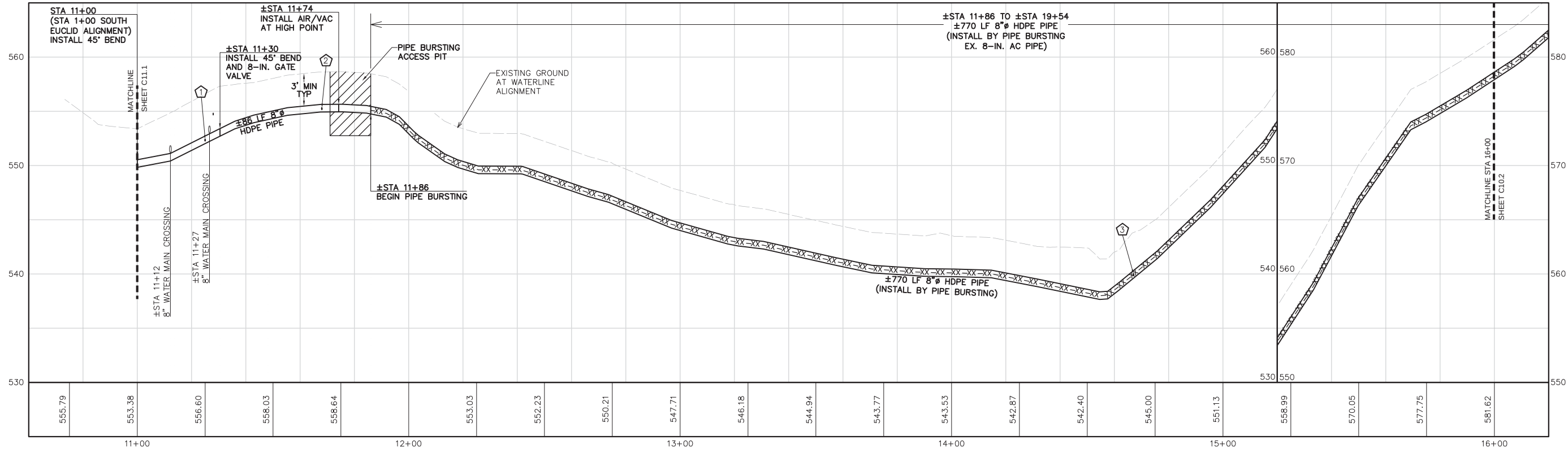
PROFILE – COLUMBUS AVENUE / LAKEHILL LANE
