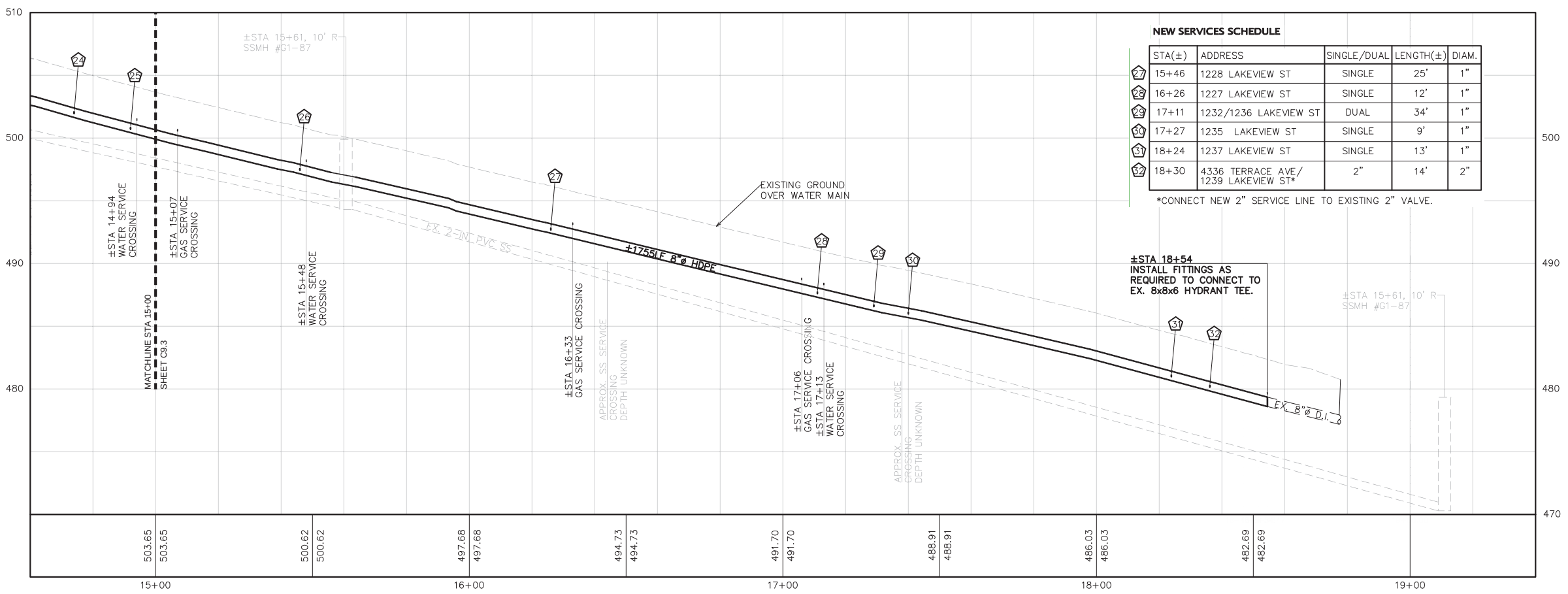
PROFILE - LAKEVIEW STREET
