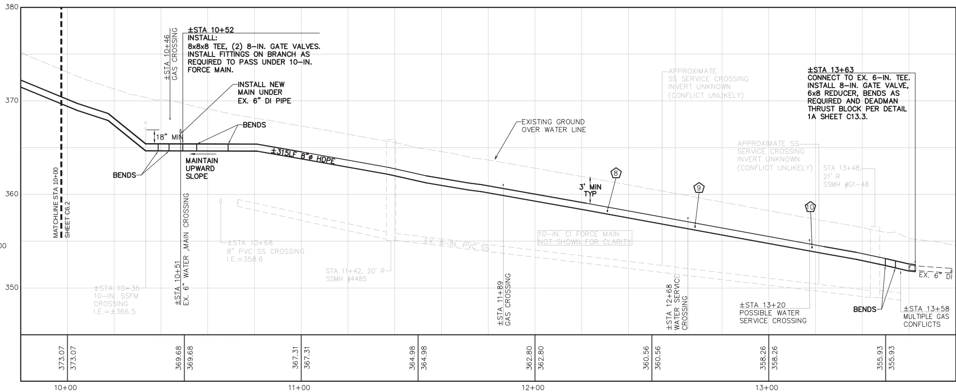
PROFILE - LAKEWAY DRIVE (EAST OF GENEVA STREET)
