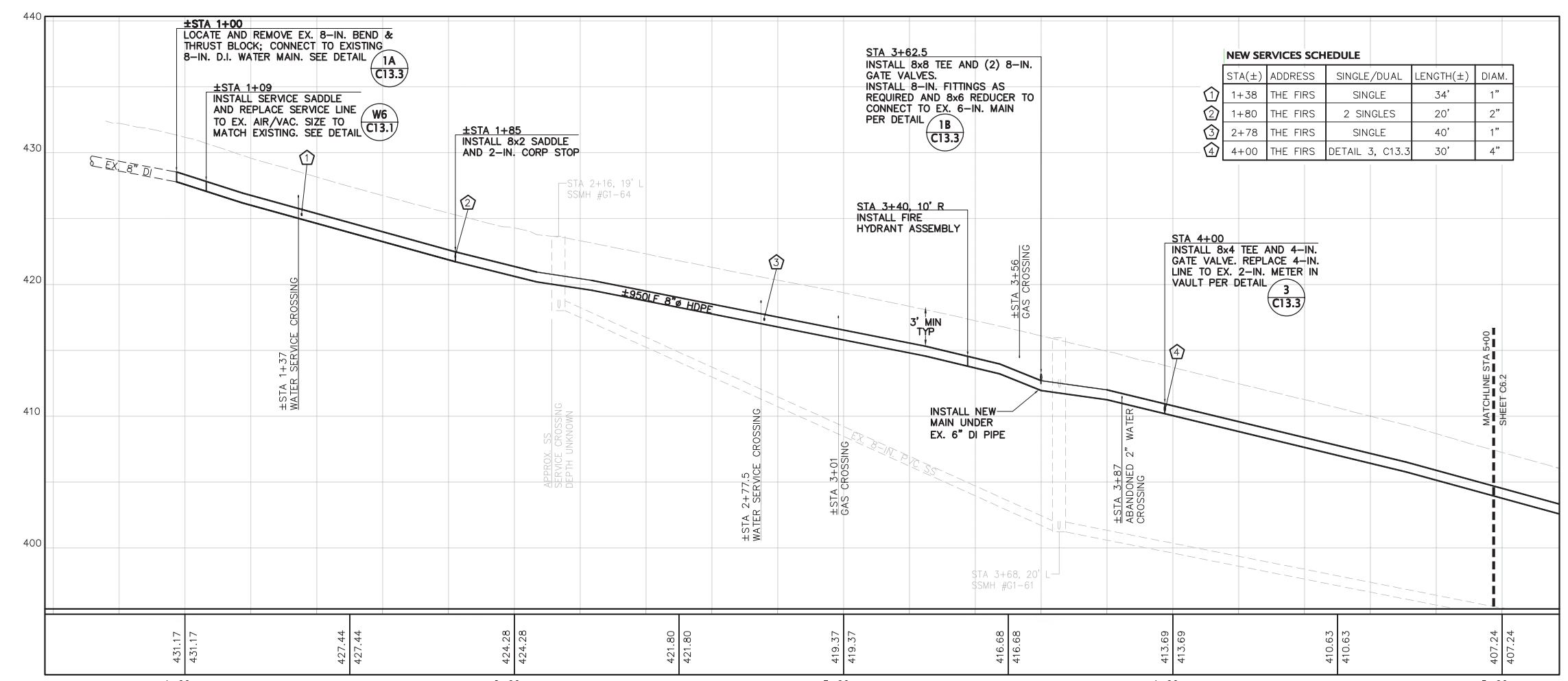
PROFILE - GENEVA STREET
